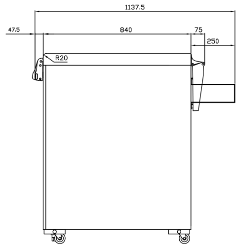
RIGHT VIEW
