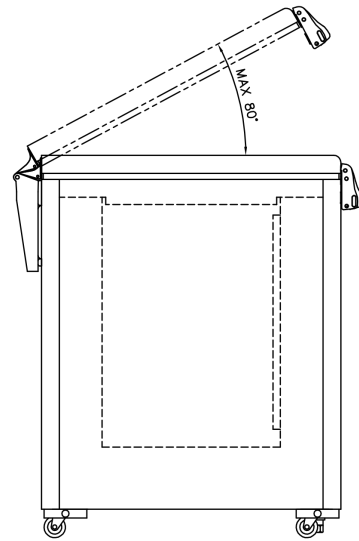
LEFT VIEW
